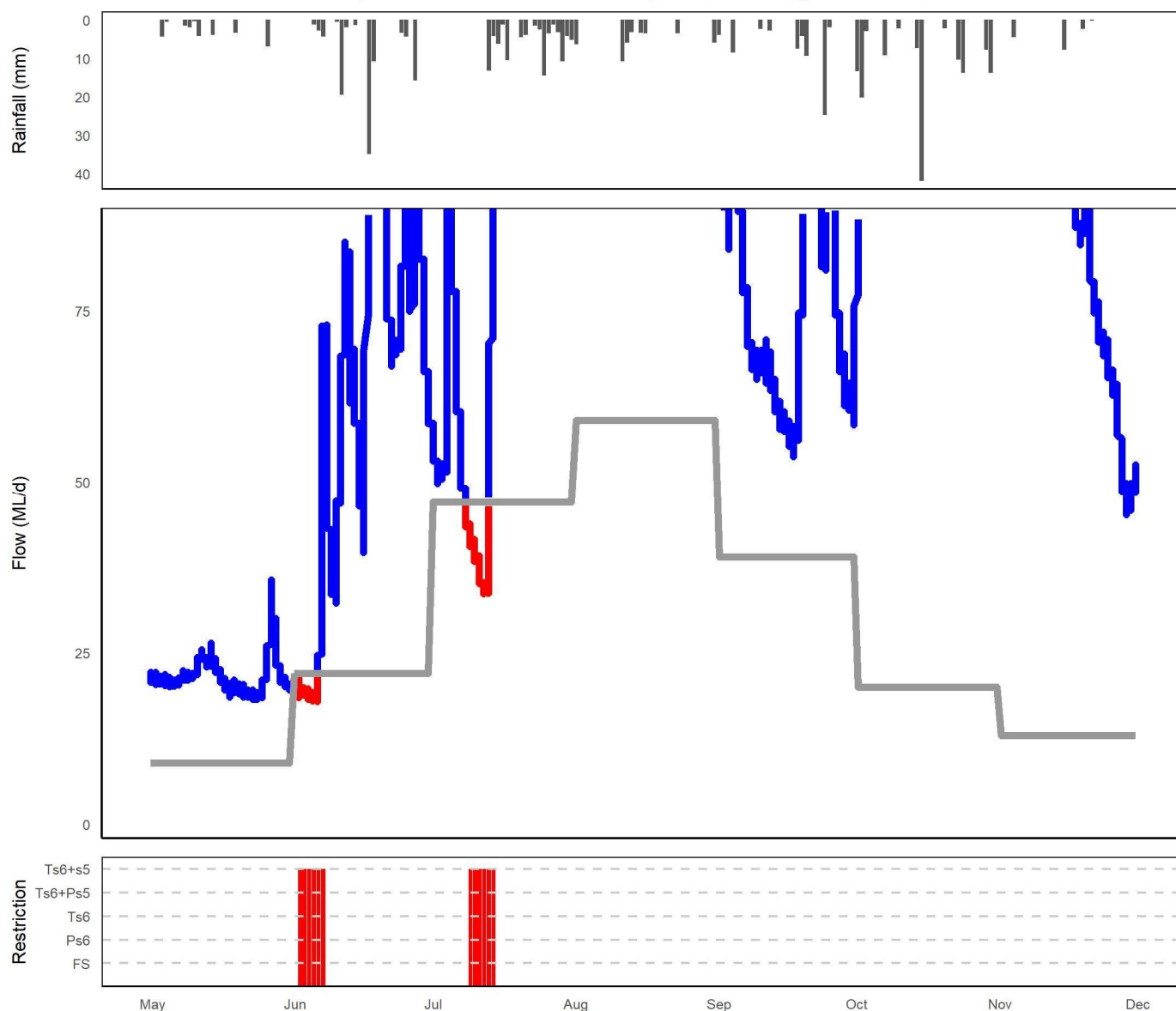
Figure 6. Summary of rainfall, low flows and restrictions in the Boobyalla River catchment during winter (May-November) 2021. Top plot: daily rainfall (Tomahawk (Carisbrooke) BoM site). Middle plot: instantaneous flow (<80 ML/d) Boobyalla River upstream Campbell Creek station (compliance flow site). Bottom plot: days when restrictions were in place.
