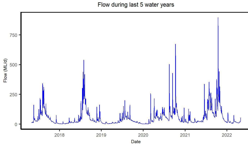
Figure 3 Mean daily flow in the Boobyalla River upstream Campbell Creek streamflow gauging station for the last five years.
