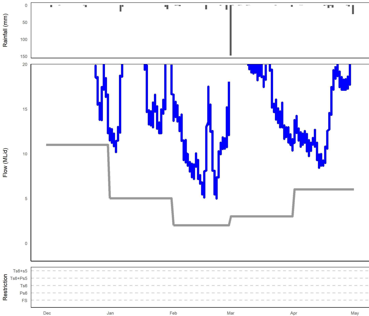
Figure 7. Summary of rainfall, low flows and restrictions in the Boobyalla River catchment during summer 2021/22 (Dec-April). Top plot: daily rainfall (Tomahawk (Carisbrooke) BoM site). Middle plot: instantaneous flow (<20 ML/d) Boobyalla River upstream Campbell Creek station (compliance flow site). Bottom plot: days when restrictions were in place.
