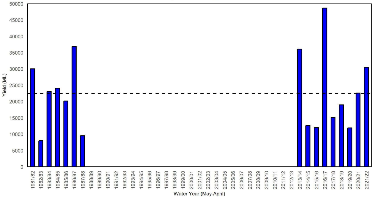
Figure 2. Yields in the Boobyalla River upstream Campbell Creek streamflow gauging station. Water years with <95% of the daily flow record available are excluded. The long-term mean yield is shown as the dashed horizontal black line (22,500 ML).
