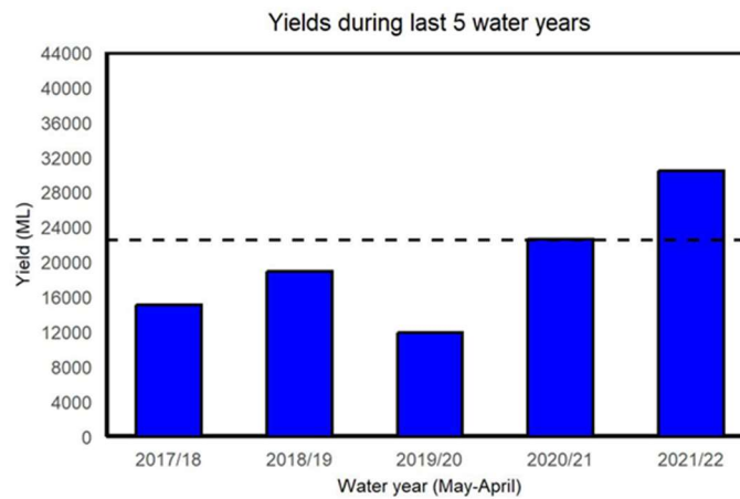
Figure 4. Yields in the Boobyalla River upstream Campbell Creek streamflow gauging station for the last five years. The long-term mean yield is shown as the dashed horizontal black line (22,500 ML).
