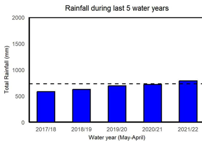
Figure 5. Total rainfall at the Tomahawk (Carisbrooke) BoM weather station during the last five water years. The long-term (1965-2021) mean total rainfall (730 mm) is shown as the black horizontal dashed line.
