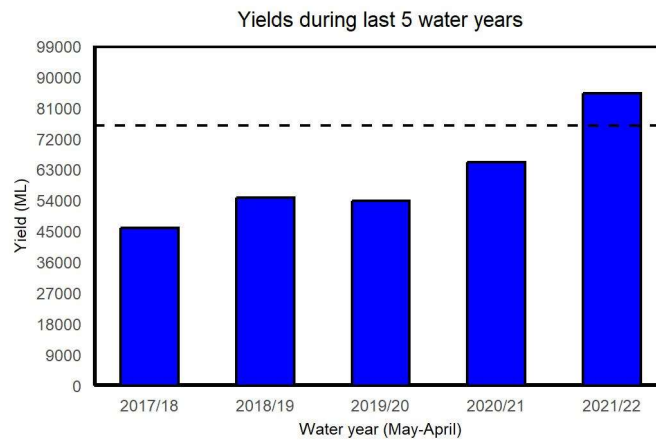
Figure 4. Yields in the Great Forester River at the Forester Road streamflow gauging station for the last five years. The long-term mean yield is shown as the dashed horizontal black line (75,700 ML).
