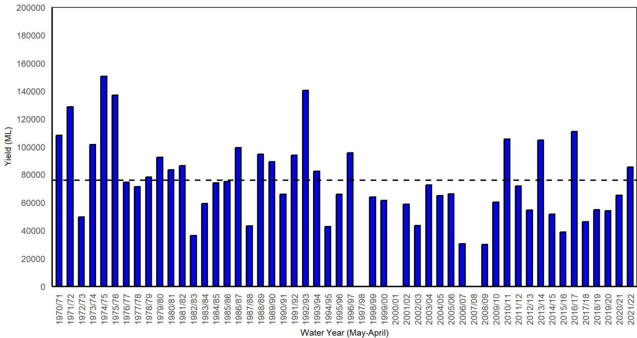
Figure 2. Yields in the Great Forester River at the Forester Road streamflow gauging station. Water years with <95% of the daily flow record available are excluded. The long-term mean yield is shown as the dashed horizontal black line (75,700 ML).
