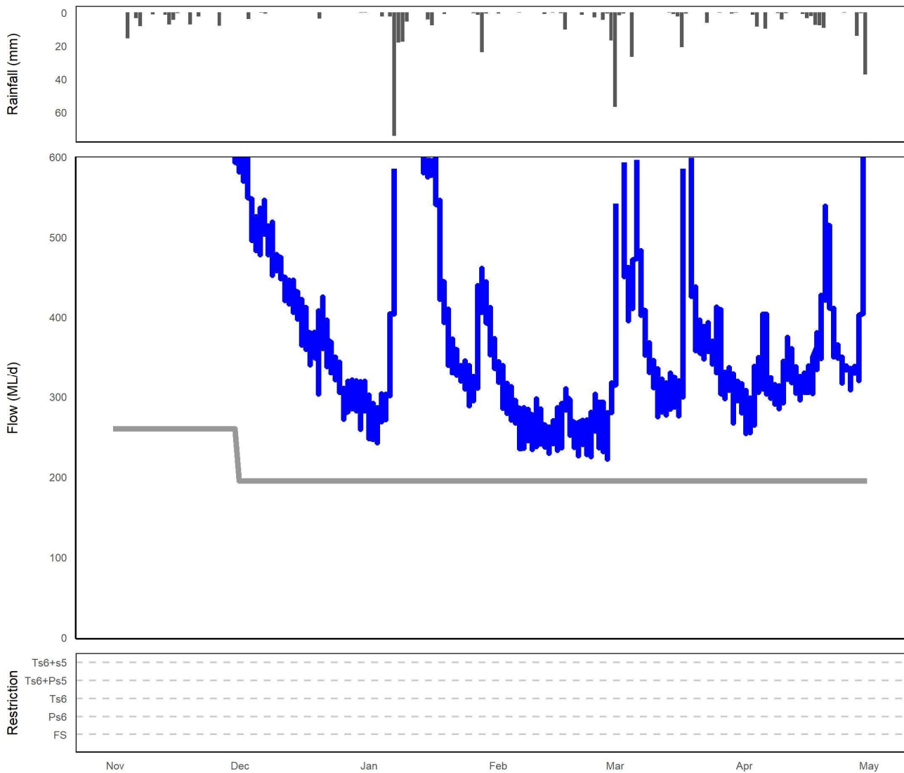
Figure 7. Summary of rainfall, low flows and restrictions in the Mersey River catchment during summer 2021/22 (Nov-April). Top plot: daily rainfall (Sheffield School Farm BoM site). Middle plot: instantaneous flow (<600 ML/d) Mersey River at Shale Road (Latrobe) station (compliance flow site). Bottom plot: days when restrictions were in place.
