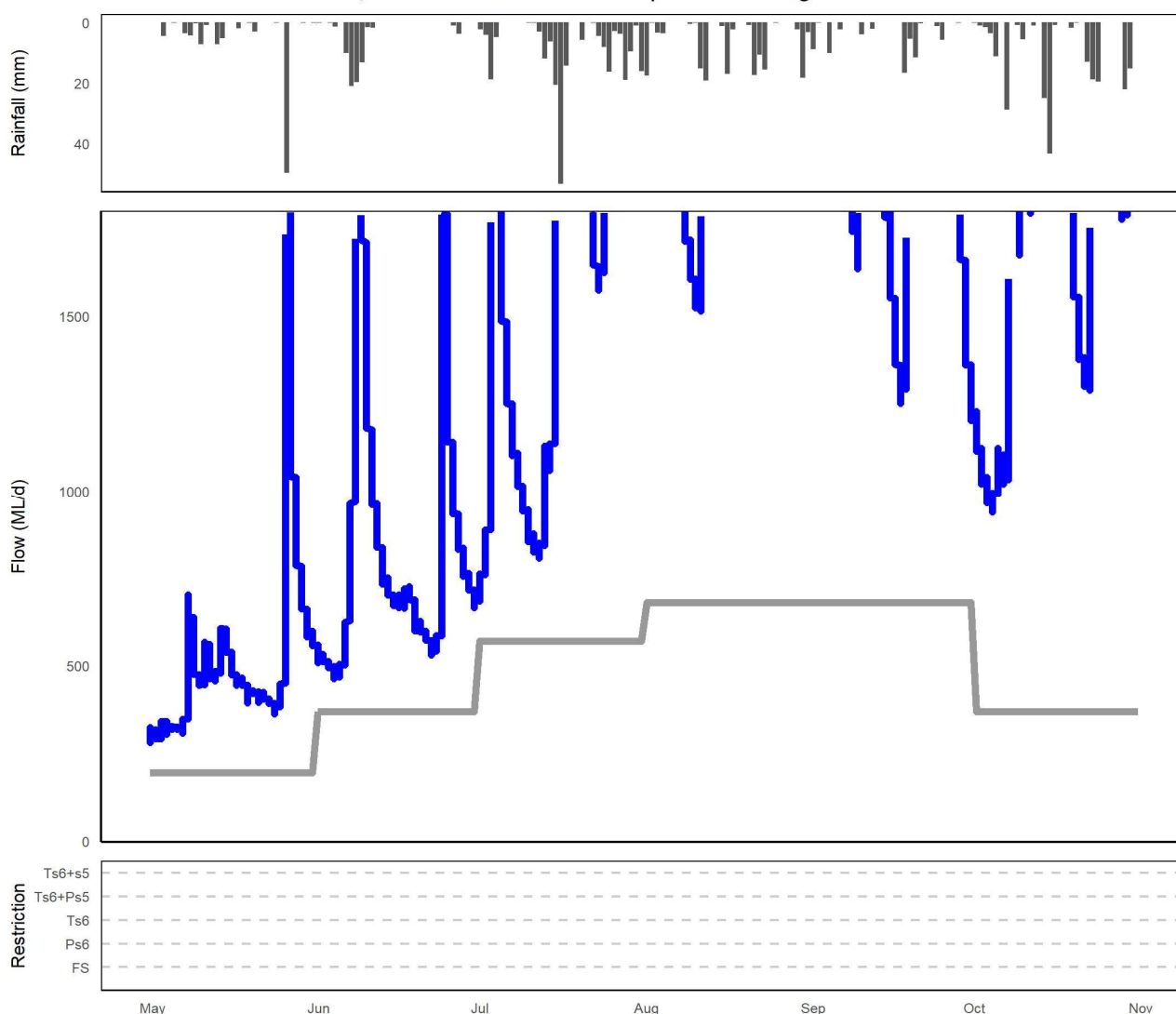
Figure 6. Summary of rainfall, low flows and restrictions in the Mersey River catchment during winter (May-October) 2021. Top plot: daily rainfall (Sheffield School Farm BoM site). Middle plot: instantaneous flow (<1800 ML/d) Mersey River at Shale Road (Latrobe) station (compliance flow site). Bottom plot: days when restrictions were in place.
