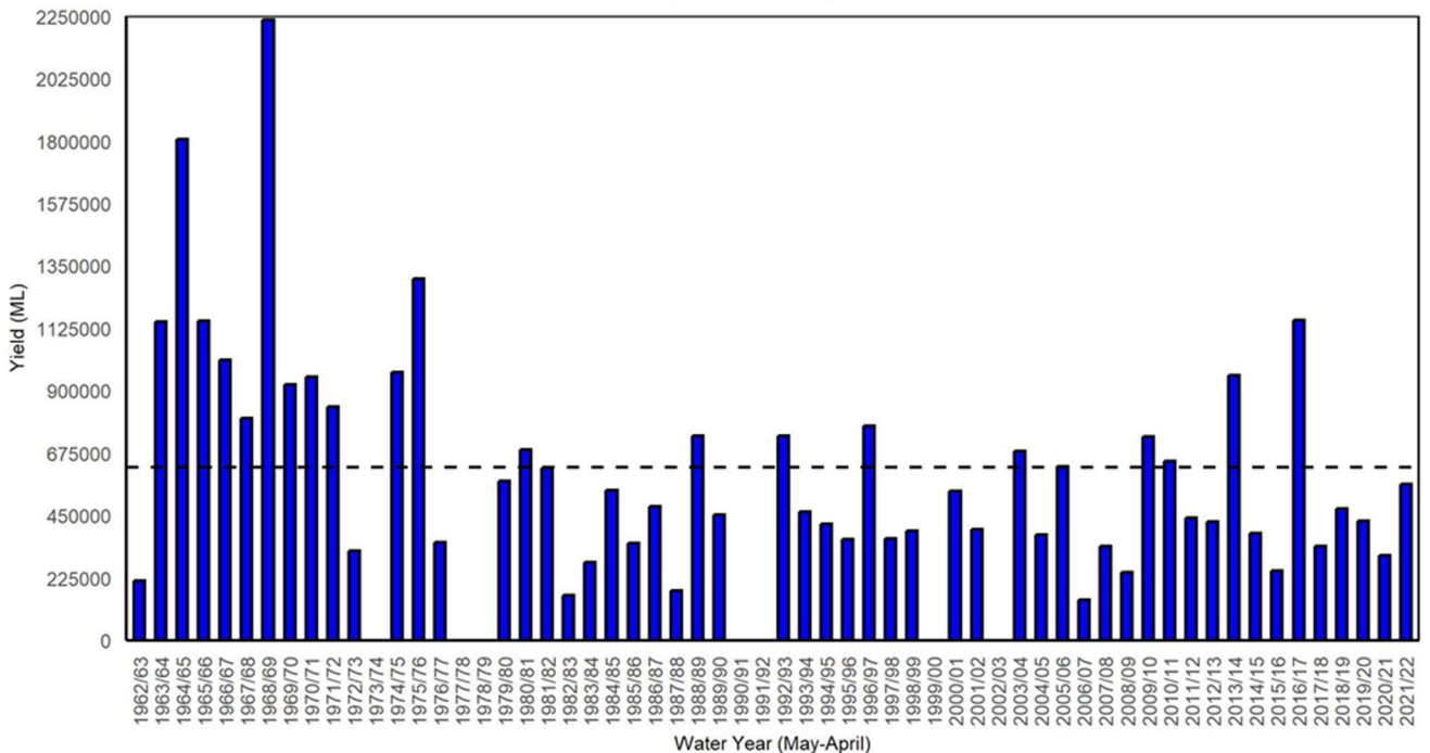
Figure 2. Yields in the Mersey River at Shale Road (Latrobe) streamflow gauging station. Water years with <95% of the daily flow record available are excluded. The long-term mean yield is shown as the dashed horizontal black line (623,800 ML).
