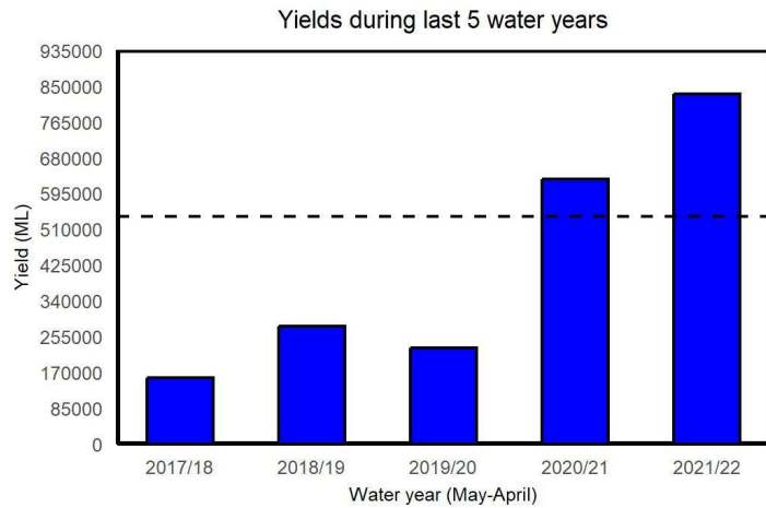
Figure 4. Yields in the South Esk River at Llewellyn streamflow gauging station for the last five years. The long-term mean yield is shown as the dashed horizontal black line (540,000 ML).
