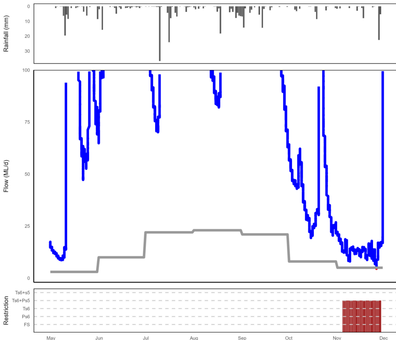
Figure 10. Summary of rainfall, low flows and restrictions in the St Pauls catchment during winter (May-November) 2024.
