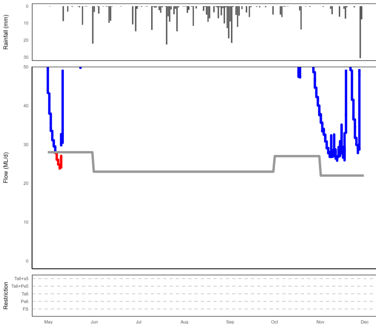
Rainfall, low flows and restriction periods during winter 2024/2025
