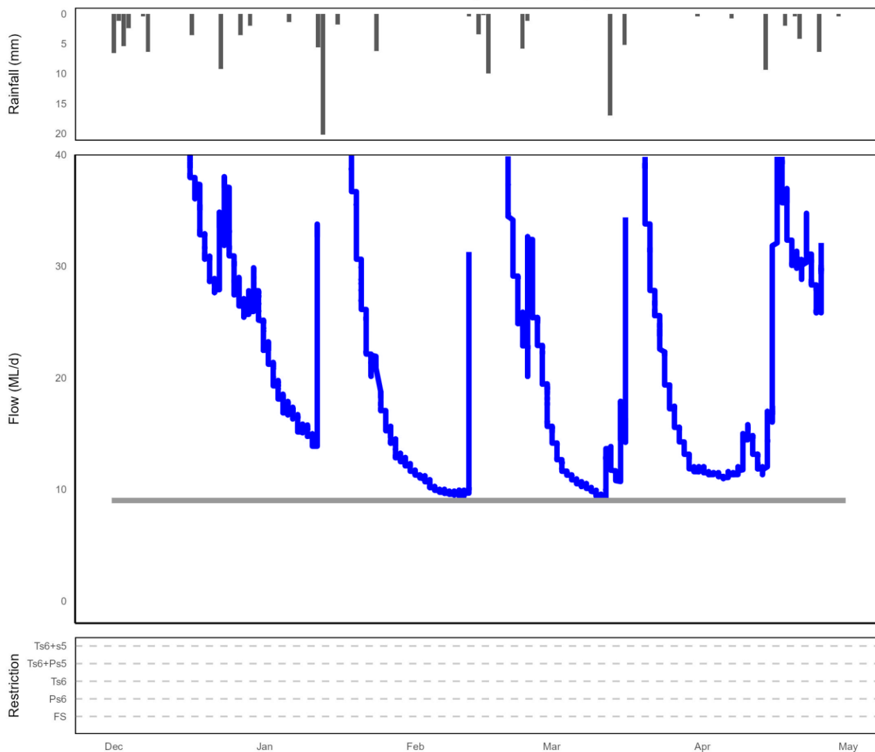
Rainfall, low flows and restriction periods during summer 2024/2025
