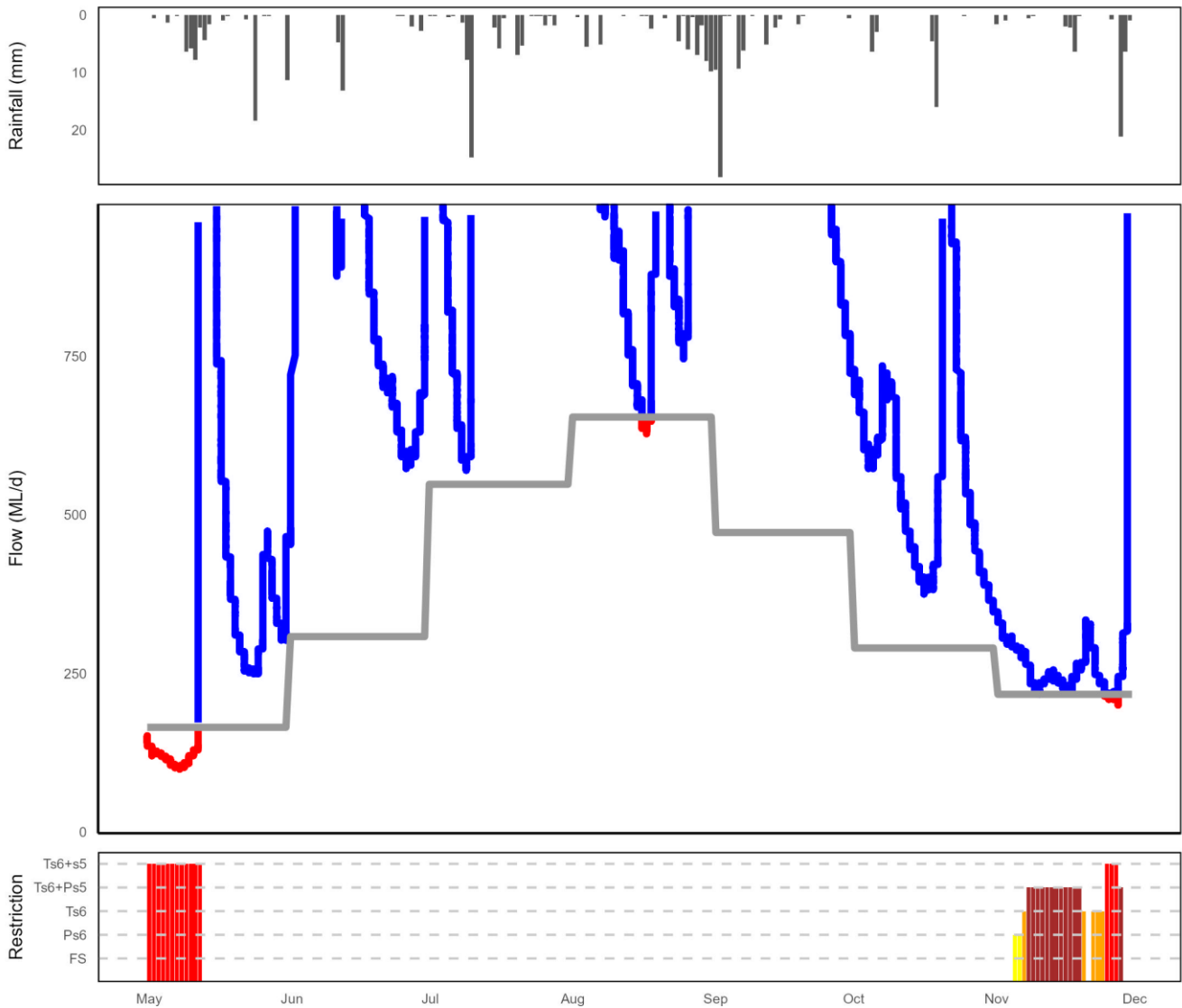
Figure 8. Summary of rainfall, low flows and restrictions in the South Esk catchment during winter (May-November) 2024.
