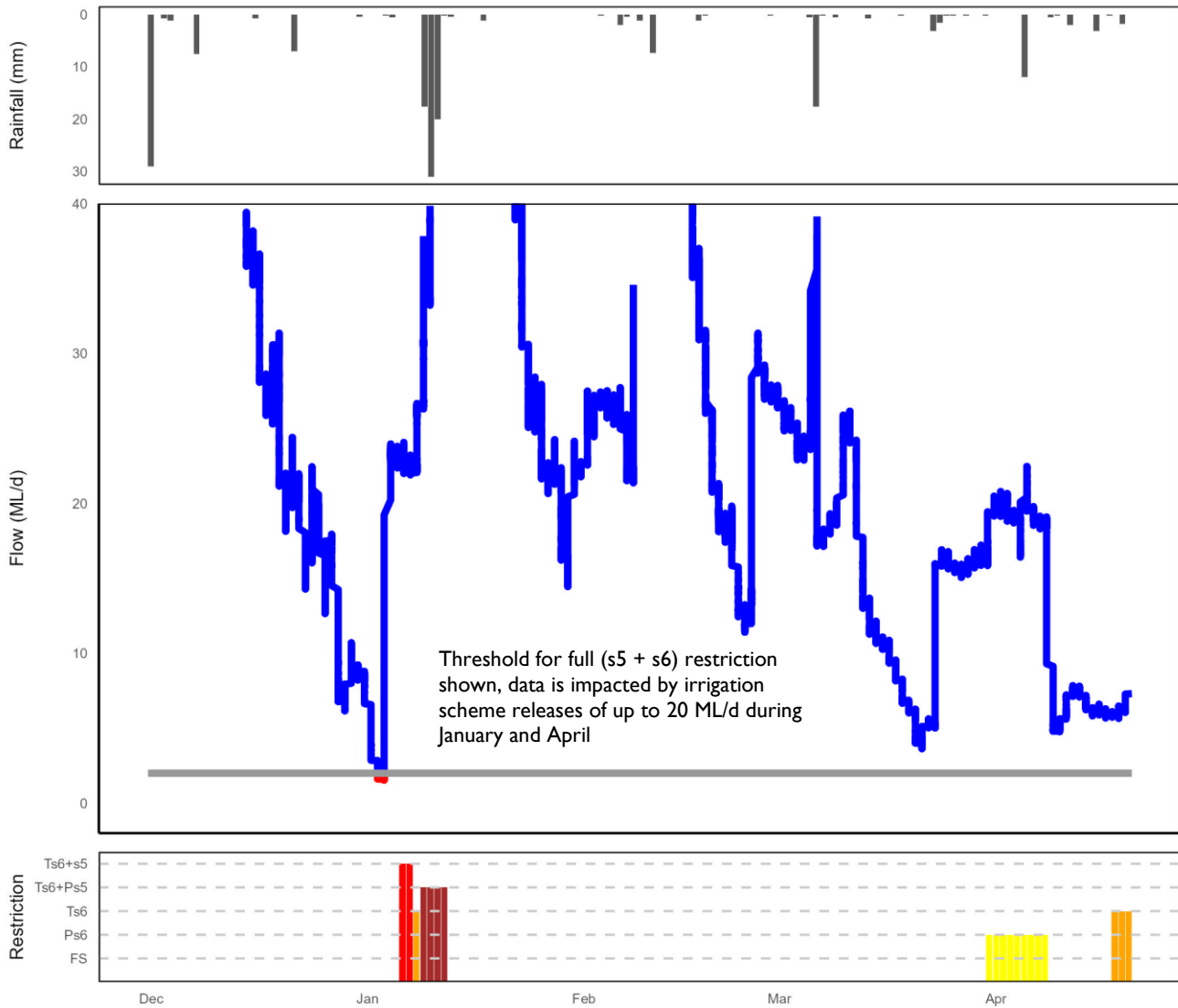
Figure 11. Summary of rainfall, low flows and restrictions in the St Pauls catchment during summer 2024/25 (Dec-April).
