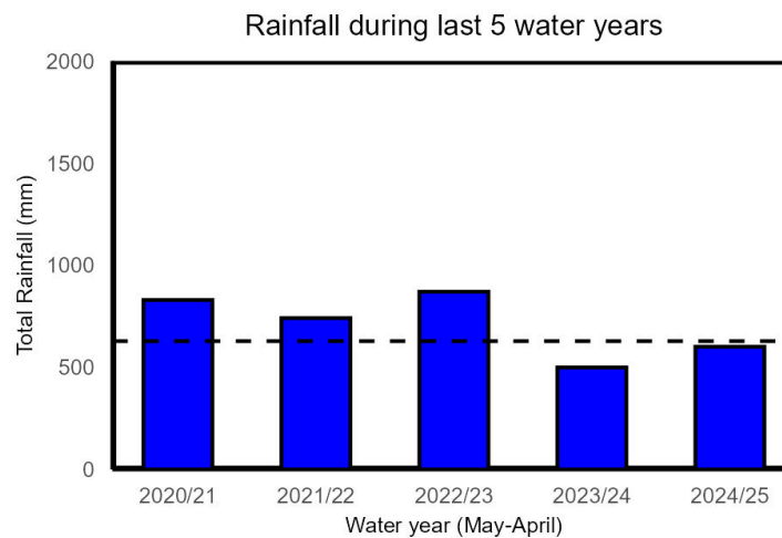
Figure 7. Total rainfall at the Mathinna (Fingal Rd) BoM weather station during the last five water years. The long-term (1970-2025) mean total rainfall (628 mm) is shown as the black horizontal dashed line
